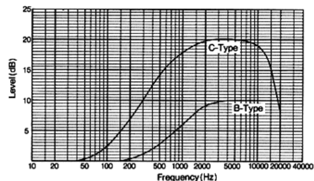
Frequency Response and Noise Spectrum Analysis
