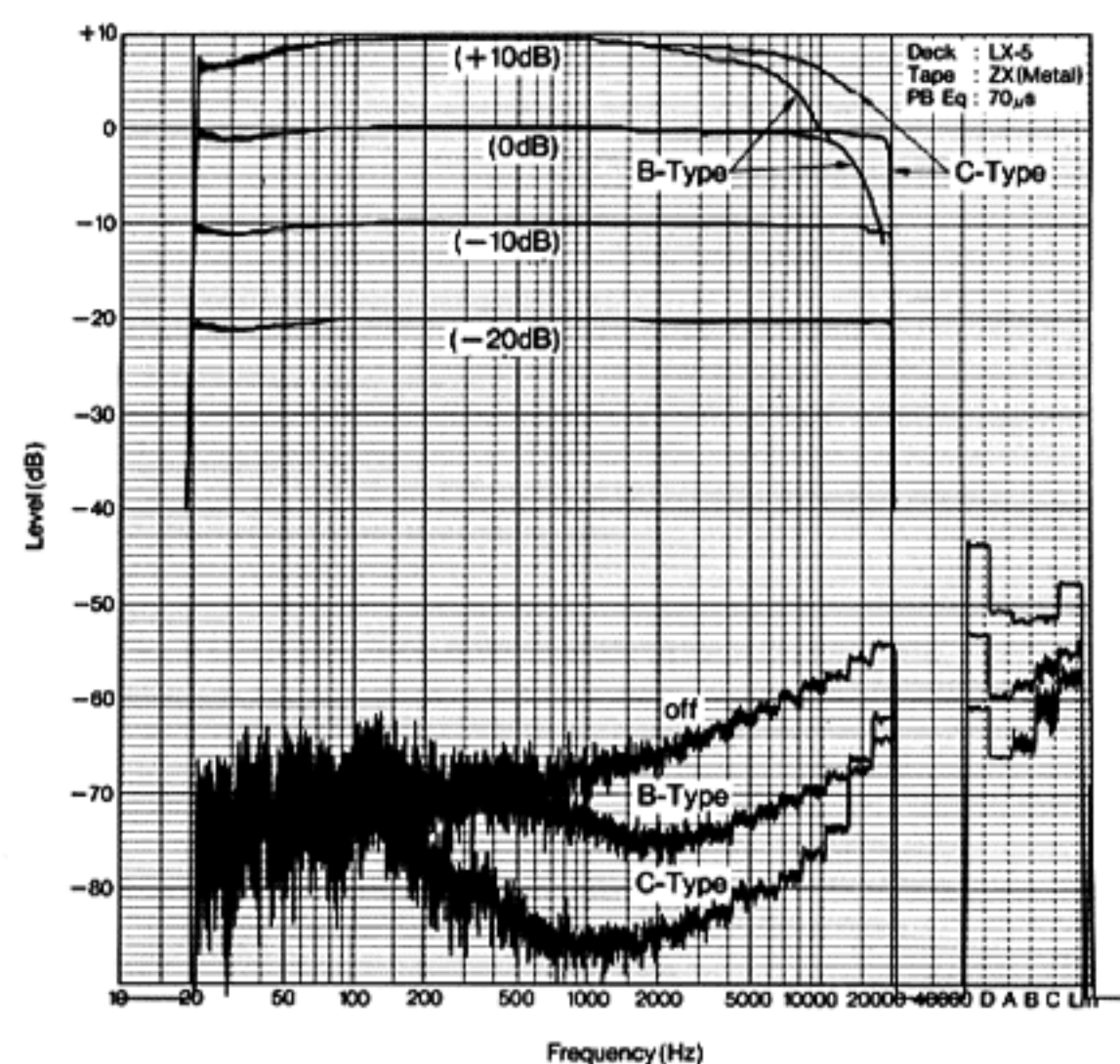
Frequency Response and Noise Spectrum Analysis
